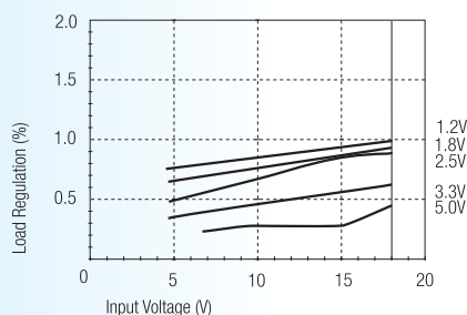
R-52xx / R-55xx Input Voltage Load Regulation VS Vin
