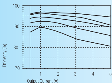
R-53xx / R-54xx / R-55xx Output Current Efficiency vs I out (Vin = Min)
